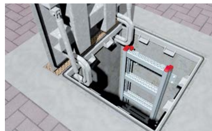
Ladder shafts
